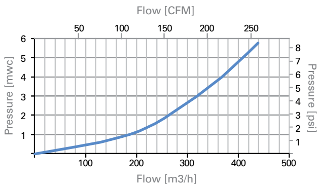
Inflow data - free air flow - 2"
