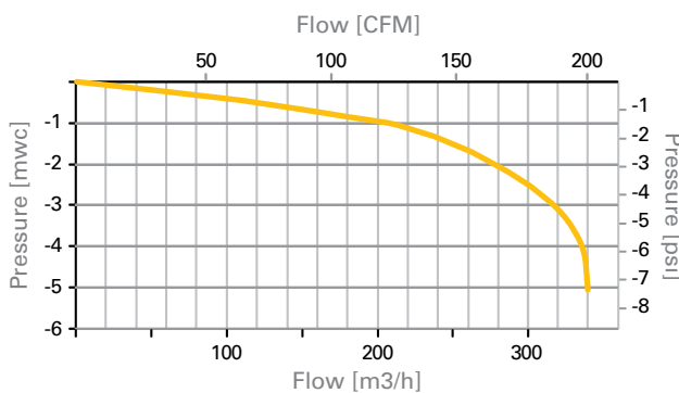
Inflow data - free air flow - 2"
