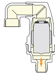
KINETIC AIR VALVE
