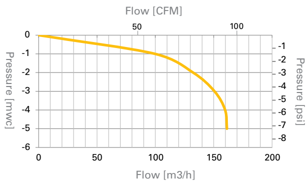
Inflow data - free air flow - 3/4", 1"
