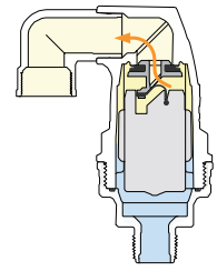
COMBINATION AIR VALVE
