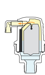
AUTOMATIC AIR VALVE
